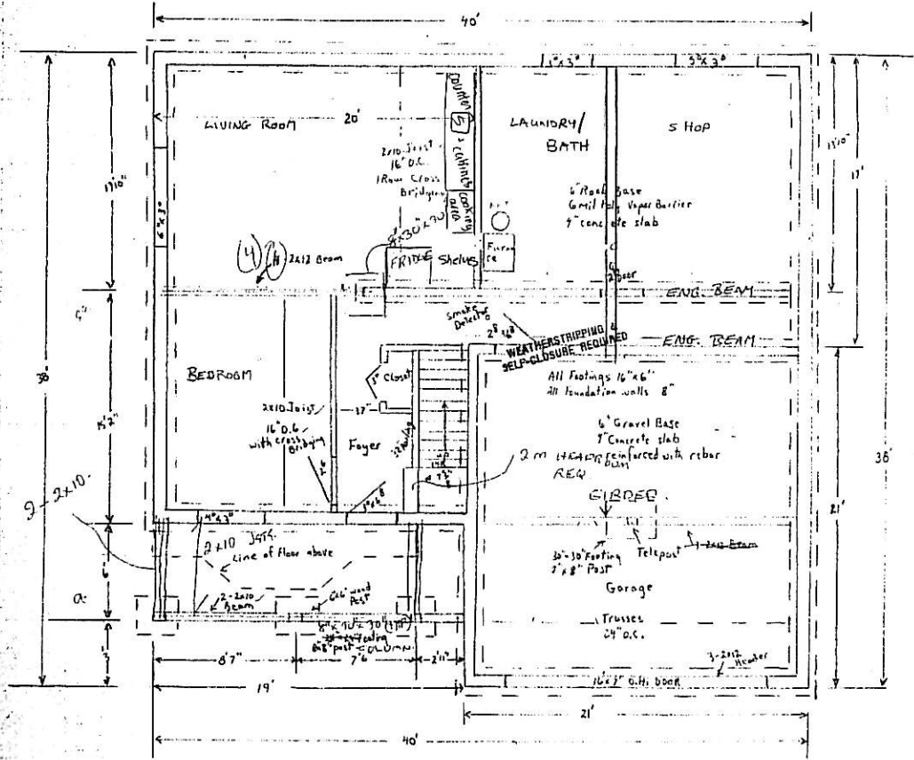
Foundation Plan
